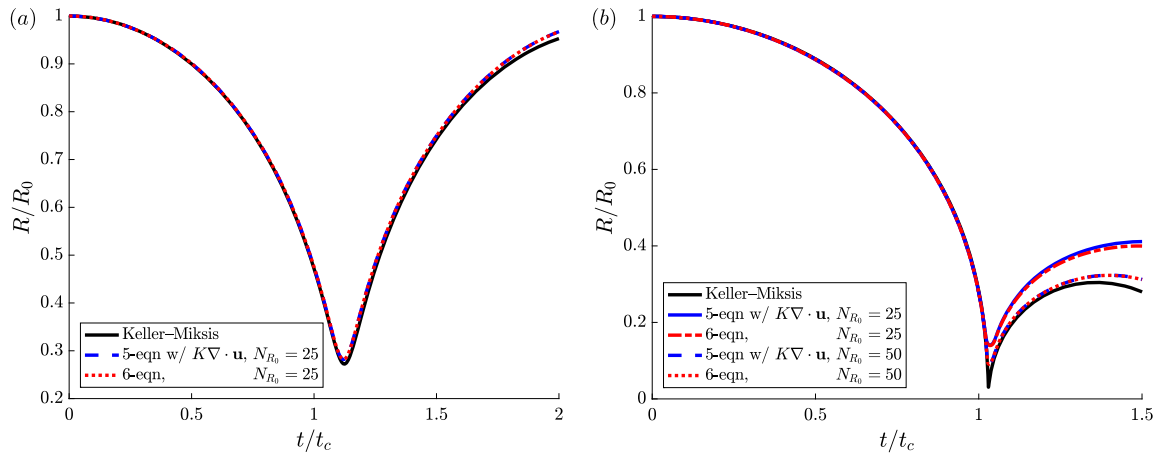
Fig. 4. Radial bubble-wall evolution for (a) p_\infty/p_b = 10 and (b) p_\infty/p_b = 1427 . Solutions are computed using WENO5. (For interpretation of the figure(s), the reader is referred to the web version of this article.)
