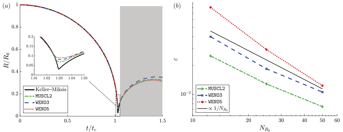
Fig. 7. Radial bubble-wall evolution for initial interface equilibrium and p_\infty/p_b = 1427 . (a) Results (fixed resolution N_{R_0} = 50 ) and (b) spatial convergence of the MUSCL2, WENO3 and WENO5 schemes.
