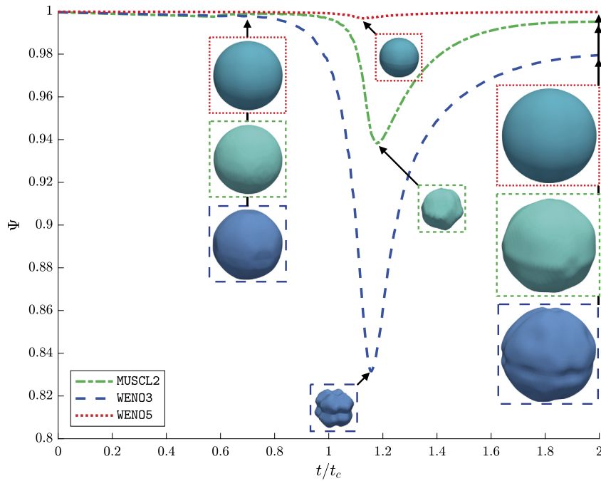
Fig. 6. Evolution of the bubble sphericity for p_\infty/p_b = 10 and N_{R_0} = 25 . Nominal bubble shapes as represented by \alpha = 0.5 isosurfaces are also shown for times t = 0.7t_c , t (R = R_{\min}) , and 2t_c .
