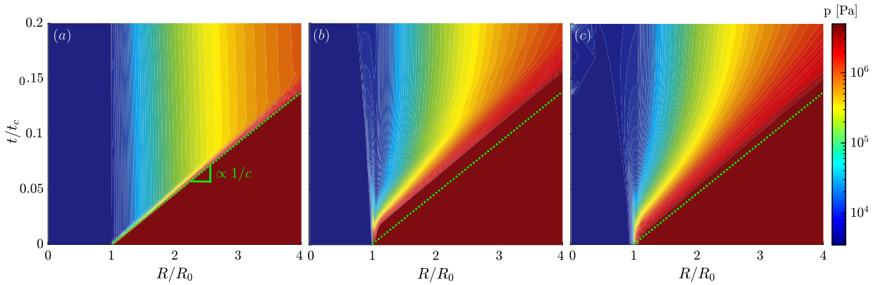
Fig. 12. Pressure in the time and radial-direction space for initial interface disequilibrium, p_\infty/p_b = 1427 and N_{R_0} = 50 . Solutions are computed using the 6-equation model with the MUSCL2 scheme for three initial configurations: (a) no initial smearing, (b) smearing on only the volume fraction \alpha , and (c) smearing on both \alpha and pressure p .
